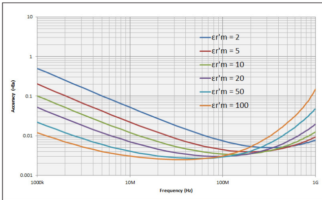
Figure 17. Dielectric loss tangent (tand) accuracy vs. frequency (at t = 1 mm, typical) 1
