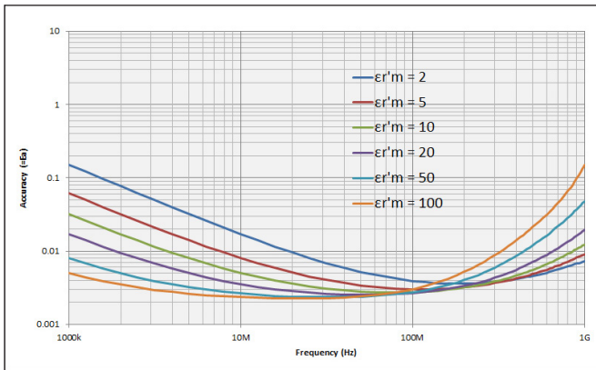
Figure 16. Dielectric loss tangent (tand) accuracy vs. frequency (at t = 0.3 mm, typical) 1
