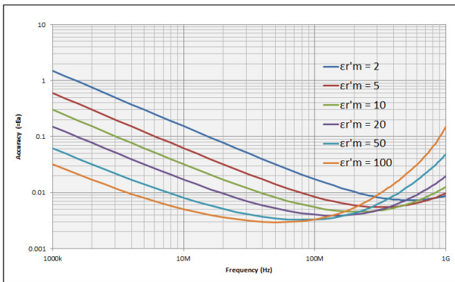
Figure 18. Dielectric loss tangent (tand) accuracy vs. frequency (at t = 3 mm, typical) 1
